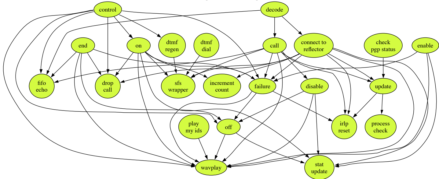
IRLP Script Call Graph http://e2.com/~ward/irlp
